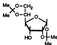
NEW 29,637-6 1,2:5,6-Di-O-isopropylidene- \alpha -D-allofuranose, 98% 1g $15.00; 5g $52.50
