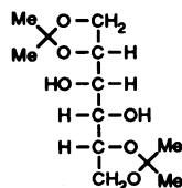
29,640-6 1,2:5,6-Di-O-isopropylidene-D-mannitol, 98% 5g $14.15; 25g $57.05
