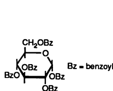
29,241-9 \alpha -D-Glucopyranose pentabenzoylate 1g $4.95; 5g $19.80
