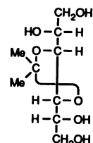
NEW 33,817-6 3,4-O-Isopropylidene-D-mannitol, 99% 1g $7.50; 5g $20.00
